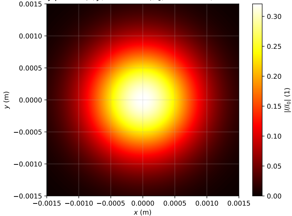
Intensity profile I(x, y, z = 3.105m)/I_0 , P_{in}=0.1P_{cr} , artificial time
